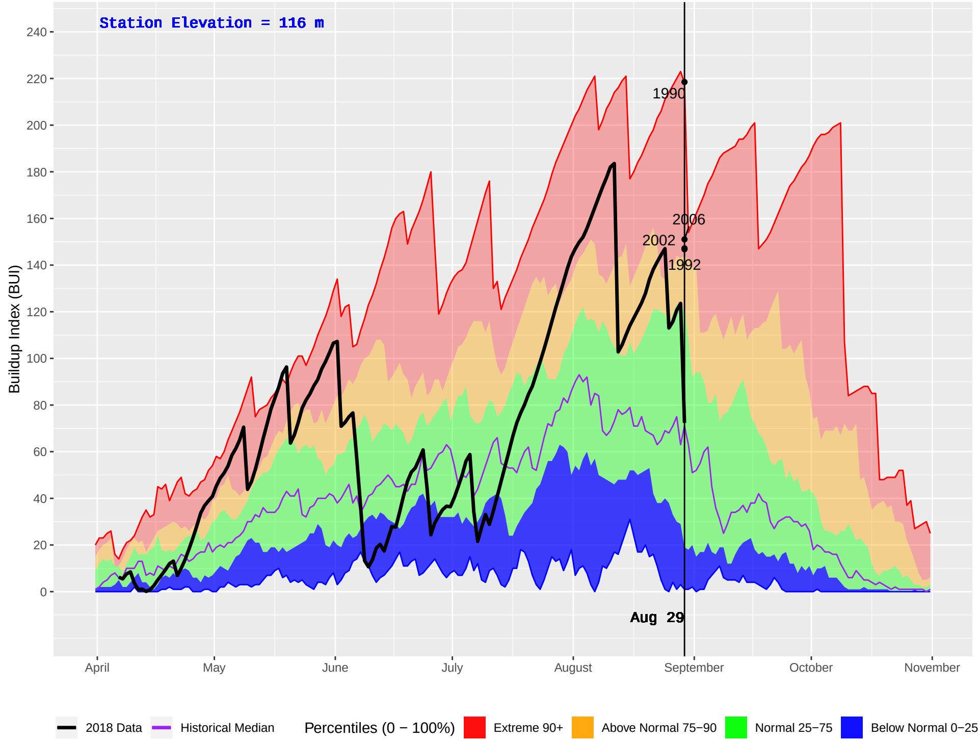
SCAR CREEK (82) : Historical (1982–2016) and Current (2018) Daily Buildup Index (BUI)
