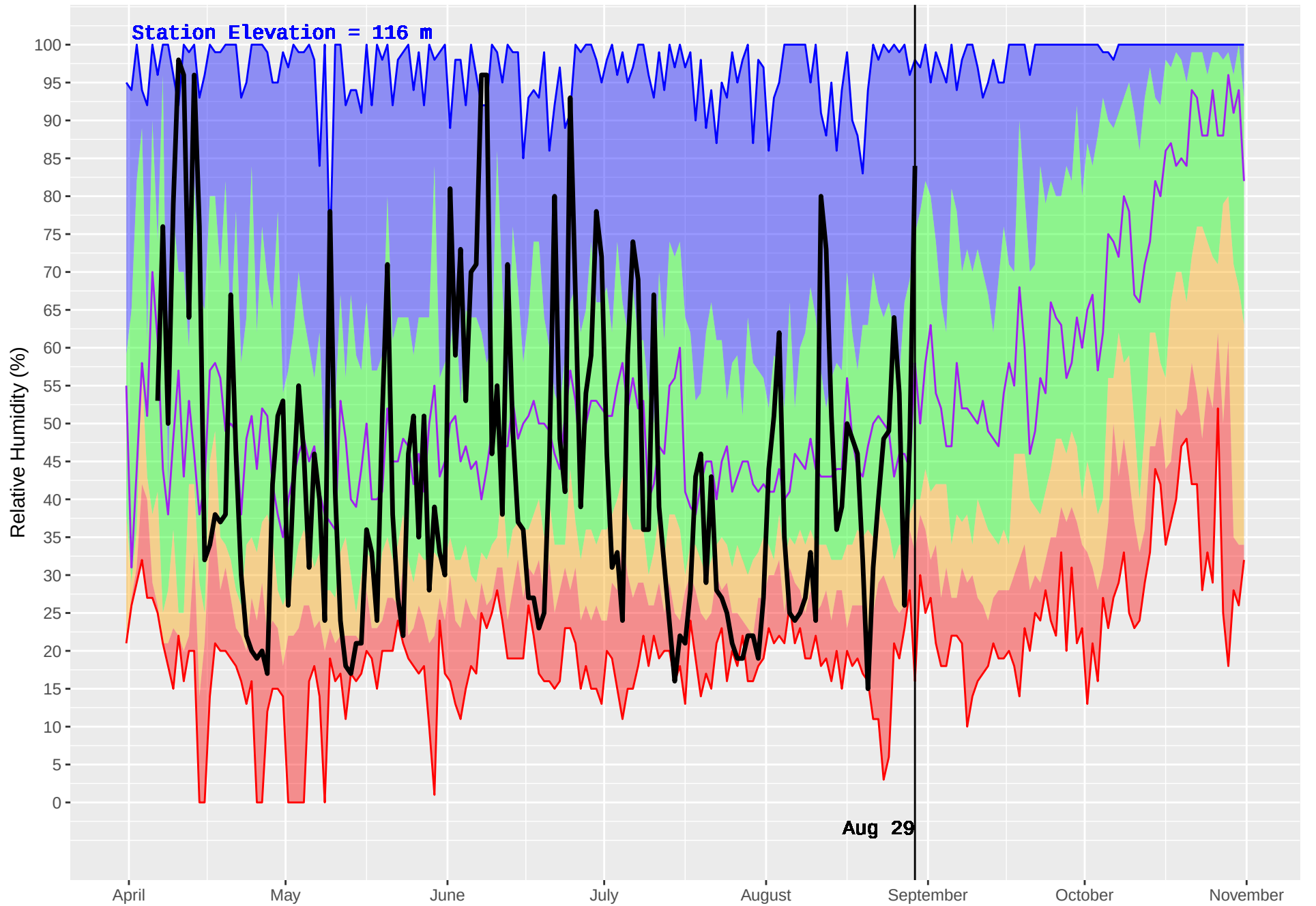
SCAR CREEK (82) : Historical (1982–2016) and Current (2018) Daily Relative Humidity
