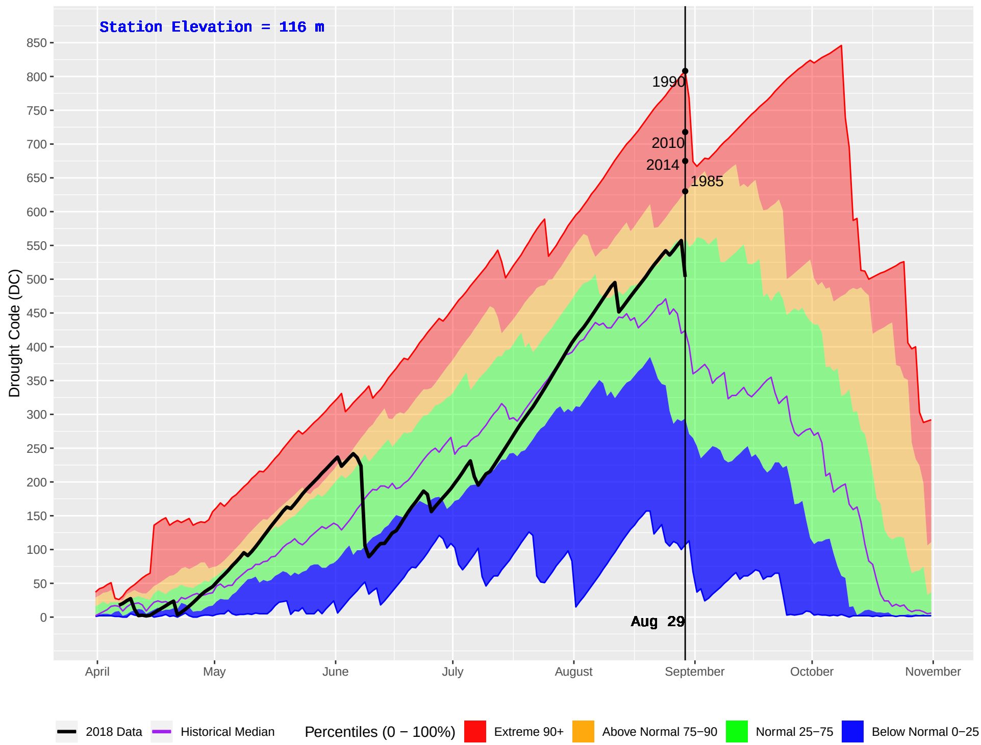
SCAR CREEK (82) : Historical (1982–2016) and Current (2018) Daily Drought Code (DC)
